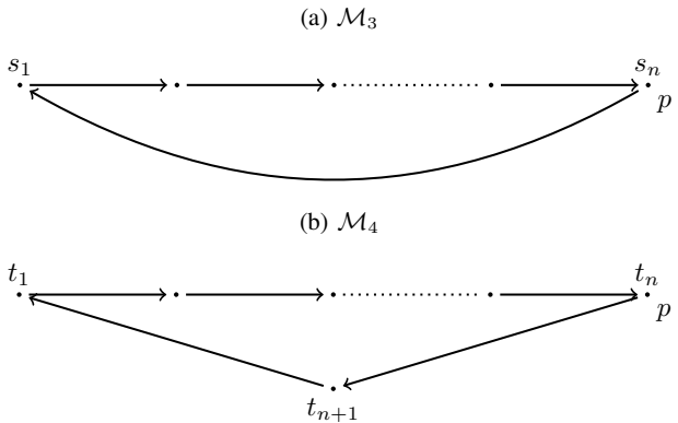
Fig. 4: Pointed transition systems (\mathcal{M}_3, s_1) and (\mathcal{M}_4, t) .
